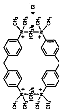
(1,4-B) 4 N 4 38C 4 -1
