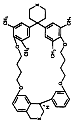
Isoquin-28C4-1 X = NC 2 H 5 + Isoquin-28C4-2 X = N(C 2 H 5 ) 2 + Cl - (+)
