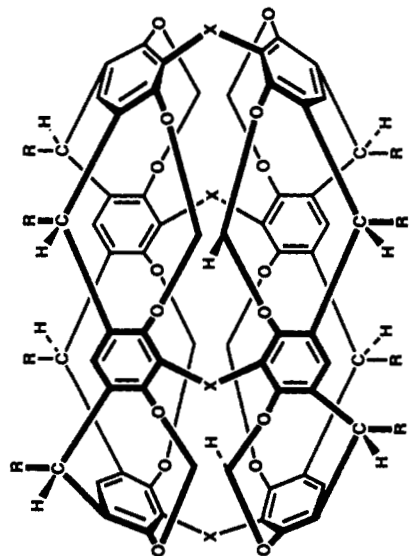
Carcerand-2 R = CH_2CH_2C_6H_5 X = CH_2SCH_2 Carcerand-3 R = CH_2CH_2C_6H_5 X = CH=N[1,3-C_6H_4]N=CH
