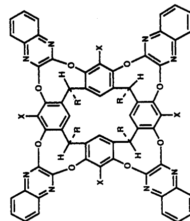
Cavitiand-2 R = C 2 H 5
