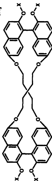
Nap 2 32C4-1 X = CH 2 CH 2 N(C 2 H 5 ) 2 + Cl - (SS)
