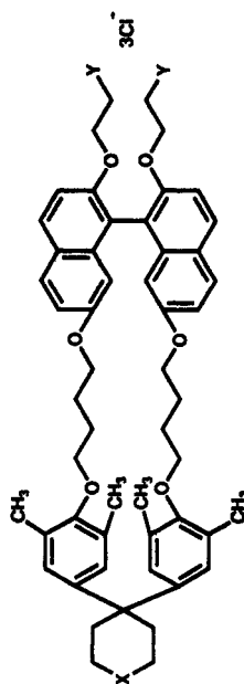
Nap 2 (1,4-B) 2 30C4-1 X = N(C 2 H 5 ) 2 + ; Y = 1,4-C 6 H 4 Nap 2 (1,4-B) 2 30C4-2 X = N(C 2 H 5 ) 2 + ; Y = 1,4-C 6 H 4 Nap 2 (1,4-B) 2 30C4-3 X = N(C 2 H 5 ) 2 + ; Y = 1,4-C 6 H 4 Y = N(C 2 H 5 ) 2 + (racemic)
