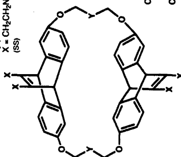
(1,4-B) 2 32C4-1 X = CO 2 CH 3 ; Y = 1,4-C 6 H 4 (1,4-B) 2 32C4-2 X = CO 2 - Cs + ; Y = 1,4-C 6 H 4 (1,4-C) 2 32C4-1 X = CO 2 - Cs + Y = 1,4-cyclohexane
