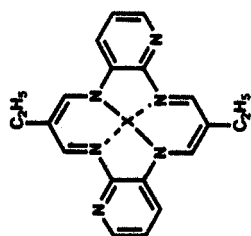
Other-20 X = Co(II) Other-21 X = Co(III)CN
