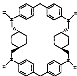
Cy 2 (1,4-B) 4 N 4 34C 4 -1
