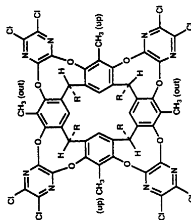
Cavitiand-9 R = C 3 H 11
