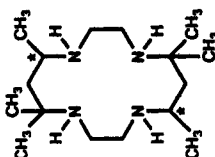
N 4 14C4-2 (racemic) N 4 14C4-3 (meso)
