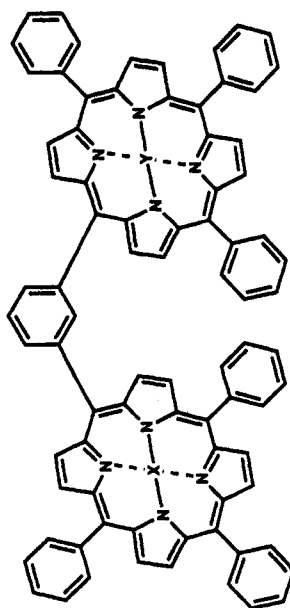
Porphyrin-73 X, Y = Fe(II) Porphyrin-74 X, Y = Co(II) Porphyrin-75 X = 2H; Y = Zn(II) Porphyrin-76 X, Y = Zn(II)
