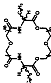
K 4 N 2 24C8-1 m = 1; n = 3 (±) K 4 N 2 24C8-2 m = 1; n = 3 (meso) K 4 N 2 24C8-3 m, n = 2
