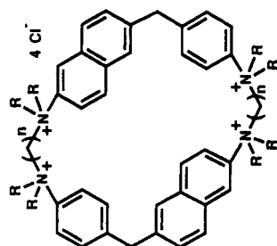
Nap 2 (1,4-B) 2 N 4 34C 4 -1
