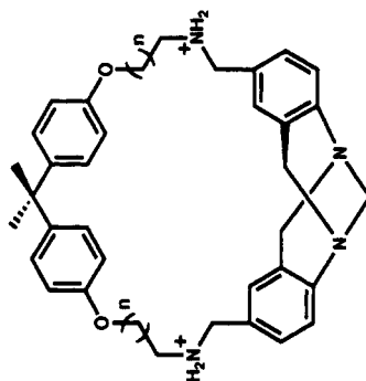
(1,4-B) 4 N 4 28C 6 -1
