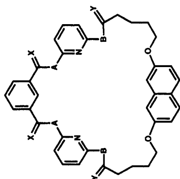
Nap(1,3-B)Py 2 N 3 32C8-1 A, Y = O; B = NH; X = H 2 Nap(1,3-B)Py 2 N 3 32C8-2 A = NH; B, X = O; Y = H 2 Nap(1,3-B)Py 2 N 3 32C8-1 A, B = NH; X, Y = O
