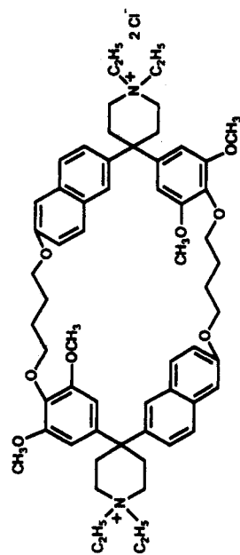
(1,4-B) 2 32C4-1 X = CO 2 CH 3 ; Y = 1,4-C 6 H 4 (1,4-B) 2 32C4-2 X = CO 2 - Cs + ; Y = 1,4-C 6 H 4 (1,4-C) 2 32C4-1 X = CO 2 - Cs + Y = 1,4-cyclohexane
