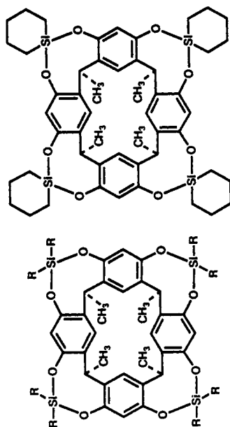
Cavitiand-2 R = C 2 H 5
