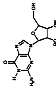
2',3',5'-tri-O-pentanylguanosine R = pentanoyl
