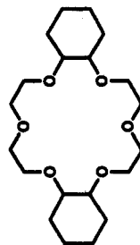
Cy 2 18C6-1 (mixture of isomers)
