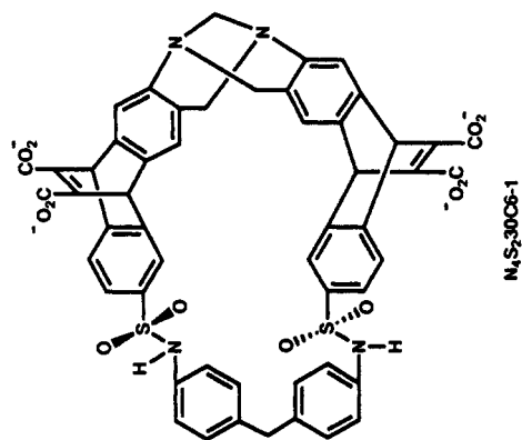
(1,4-B) 4 N 4 28C 6 -1
