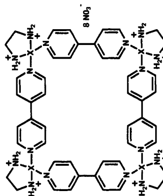
Py 6 Pd 3 36C4-1 X = Pd (III) Py 6 Pt 3 36C4-1 X = Pt (II)
